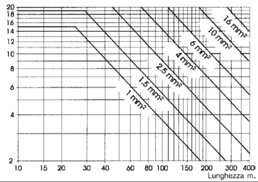
THREE-PHASE
